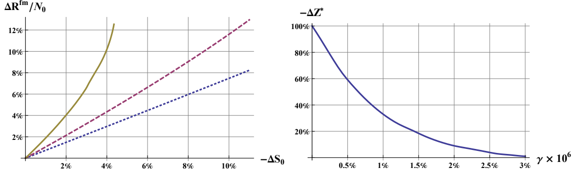
Figure 3: The graph in the left panel shows the outflow due to first movers in response to an exogenous shock on the fund’s NAV. The flow-to-performance relation depends on the liquidity of the asset held by the fund: the asset illiquidity parameter \gamma is 0.5 \times 10^{-8} (dotted line), 1.5 \times 10^{-8} (dashed line), and 2.5 \times 10^{-8} (solid line). The graph in the right panel shows the critical level \Delta Z^* as a function of the illiquidity parameter \gamma . The horizontal axis reports the price impact per $1 million. The proportion \pi of first movers is 75%.
