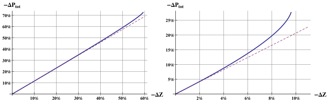
Figure 2: The graphs show the aggregate impact on market prices of an initial market shock, for \pi = 75\% (solid line) and \pi = 0 (dashed line). The asset illiquidity parameter \gamma is 0.5 \times 10^{-8} (left panel) and 2 \times 10^{-8} (right panel). These values of \gamma correspond to typical liquidity levels for corporate bonds, as reported in the empirical study by Ellul et al. (2011). The flow-performance relation \frac{\beta}{N_0} is chosen to be 0.859, consistently with the estimates in Goldstein et al. (2017). In the presence of first movers, the impact on prices grows superlinearly with the size of the shock, if the asset is illiquid.
