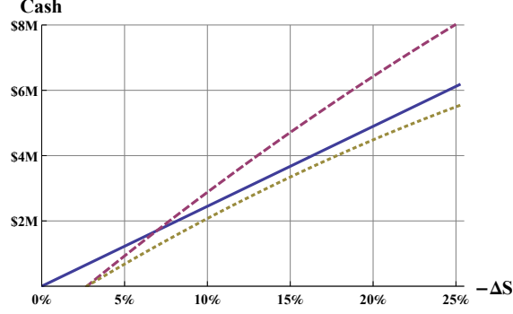
Figure 4: For each value of \Delta S , we compute R_{tot}^{fm} from equation (2.12) and Q_{tot}^{fm} from equation (2.13). The graph shows the cash owed to first movers, i.e., the right-hand side of equation (2.19), (solid line) and the cash raised by selling asset shares, i.e., the left-hand side of equation (2.19), for \gamma = 1 \times 10^{-8} (dashed line), and for \gamma = 2.5 \times 10^{-8} (dotted line). For \gamma = 2.5 \times 10^{-8} , the fund is unable to repay its redeeming investors for any value of \Delta S .
