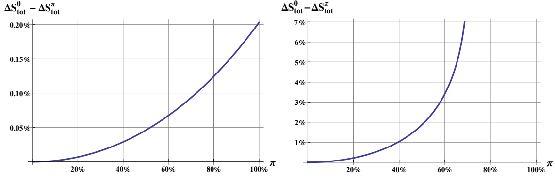
Figure 6: The graphs show the impact of first movers' redemptions on the value of a fund share, i.e., \Delta S_{tot}^0 - \Delta S_{tot}^\pi . We set the price impact parameter \gamma = 1 \times 10^{-8} (left panel), and \gamma = 2.5 \times 10^{-8} (right panel). For the larger value of \gamma , the impact diverges if \pi \geq 70\% .
