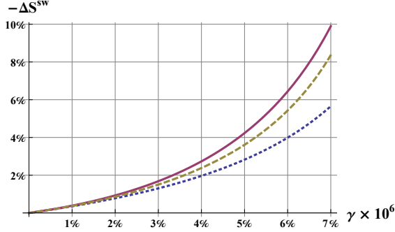
Figure 8: Comparison of the swing prices \Delta S_{both}^{sw} (dotted line), \Delta S_{loc}^{sw} (dashed line) and \Delta S_{glob}^{sw} (solid line) for different levels of illiquidity \gamma . The horizontal axis reports the price impact per $1 million. The proportion of first movers in each fund is \pi_1 = \pi_2 = 75\% .
