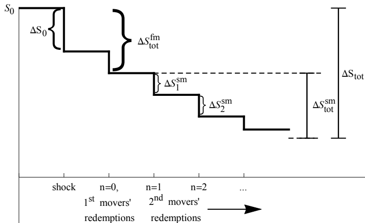
Figure 1: Timeline of the model. The initial market shock is \Delta S_0 = \Delta Z . The total drop in NAV following first-mover redemptions is \Delta S_{tot}^{fm} ; this drop triggers an initial round of second-mover redemptions, and each such round leads to further redemptions with further NAV drops \Delta S_n^{sm} .
