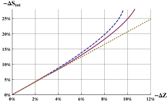
Figure 5: The graph shows the change in value of a fund share with the swing price specified in Proposition 4.3 (dotted line), without swing price (dashed line), and with a fixed NAV adjustment applied when more than 5% of investors exit the fund (solid line). The proportion \pi of first movers is 75%.
