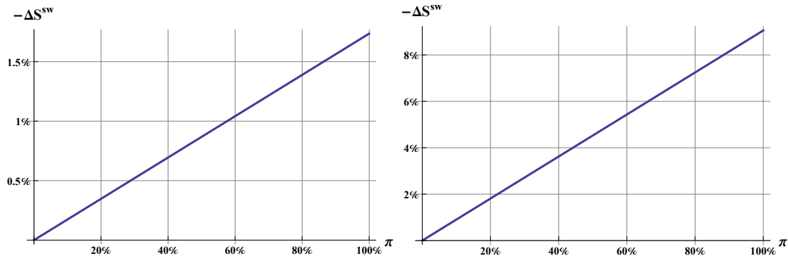
Figure 7: The swing price as a function of \pi . We set the price impact parameter \gamma = 1 \times 10^{-8} (left panel), and \gamma = 2.5 \times 10^{-8} (right panel).
