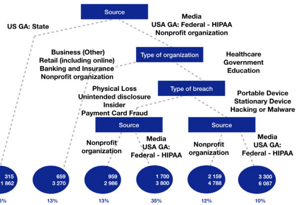
Fig. 5. Tree obtained from the CART algorithm based on the absolute loss fitted on the observations such that the variable “Number of Records” is less than u . For each leaf, the median (above) and the mean (below) are given.
