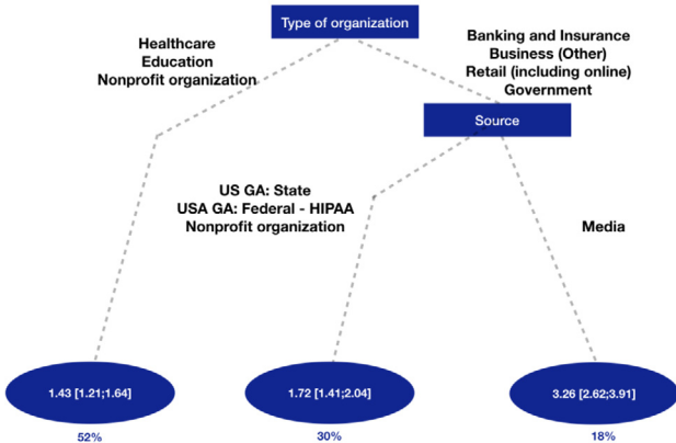
Fig. 4. Tree obtained from the CART algorithm based on the Generalized Pareto log-likelihood splitting rule (fitted on the observations exceeding the threshold u ). For each leaf, the estimates of \gamma and their 95% confidence intervals are given.
